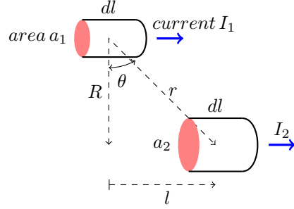
FIGURE 1. Elements q_1, q_2 in two horizontal parallel conductors one above the other, distance R apart, angular offset of angle \theta with corresponding uniform charge densities, electron drift velocities \rho_1, v_1, \rho_2, v_2 .
