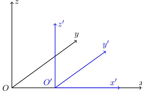
FIGURE 1. S frame black, origin O ; S' frame blue, origin O' moves with uniform velocity v along x direction.
